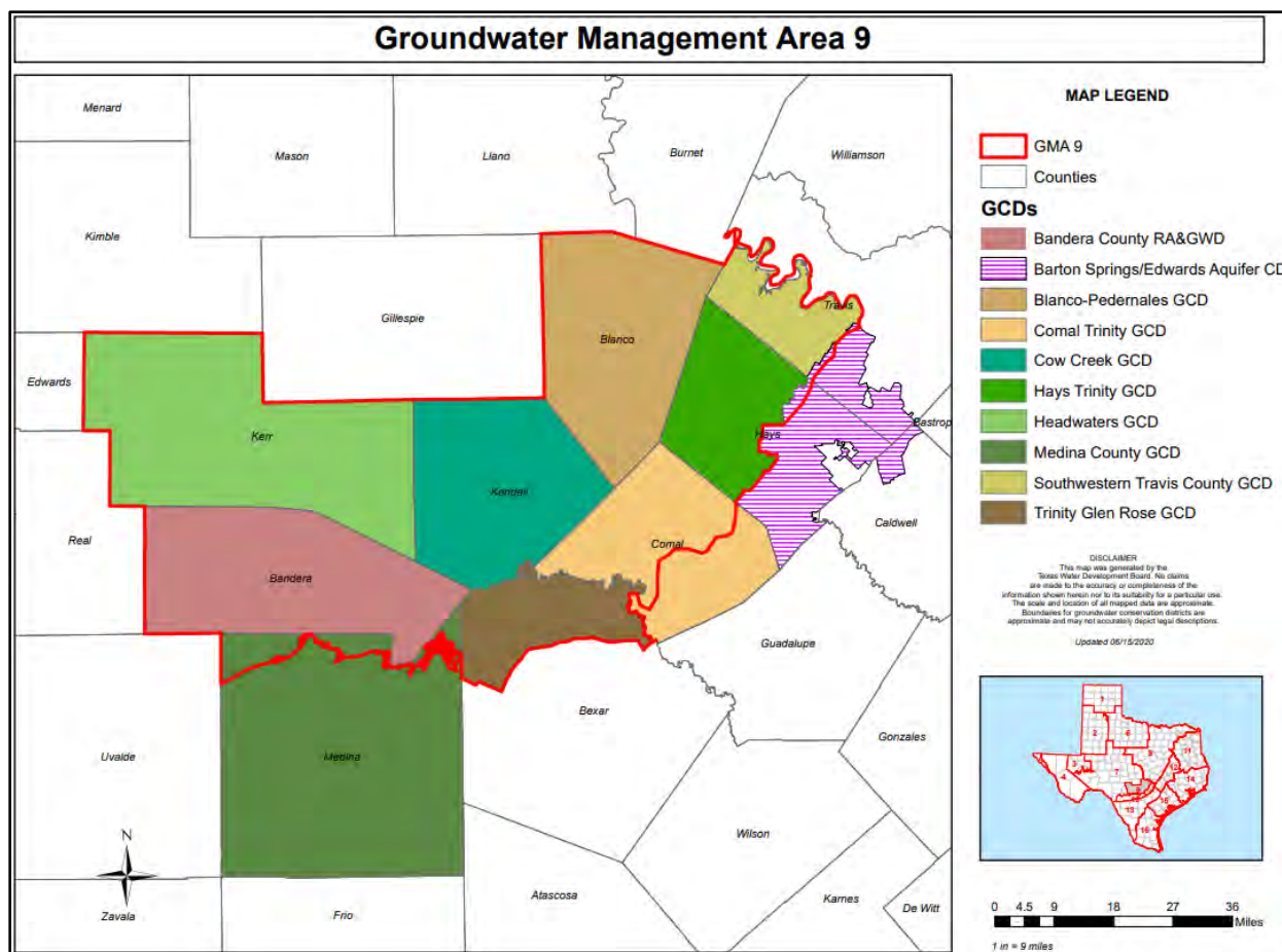
Figure 3: Map of Groundwater Management Area 9
